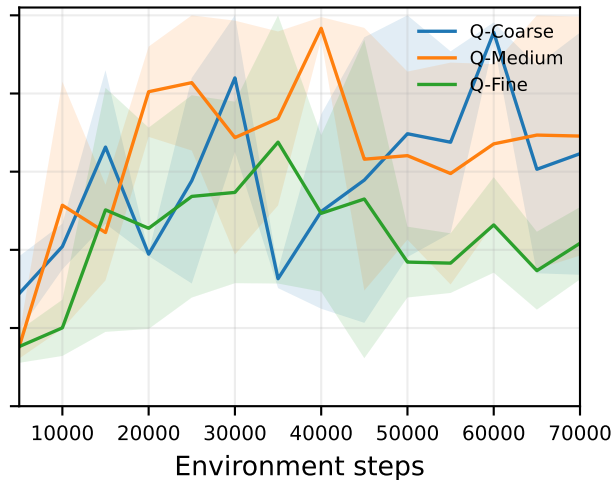
Q-Learning discretizations
