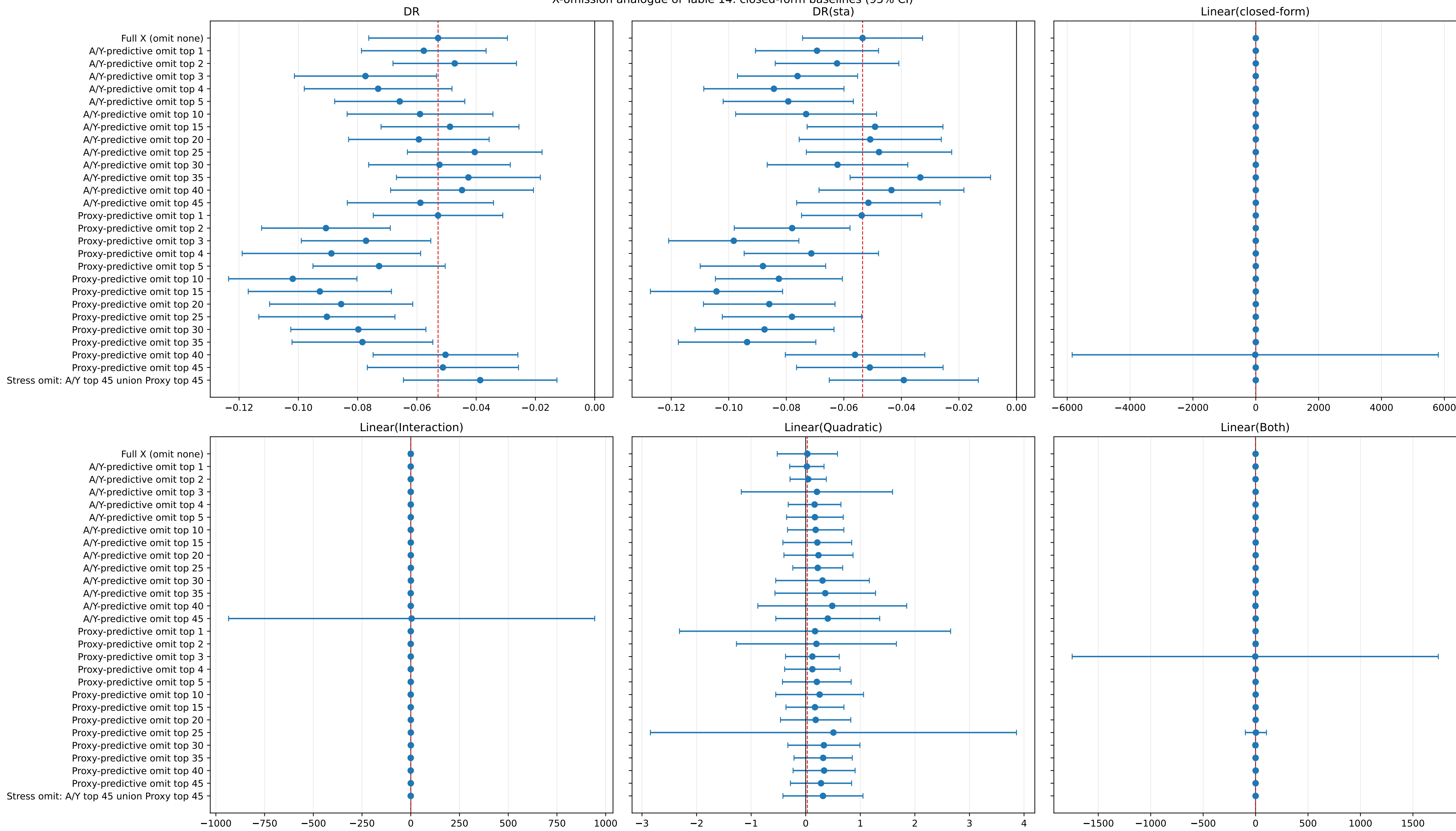
X-omission analogue of Table 14: closed-form baselines (95% CI)
