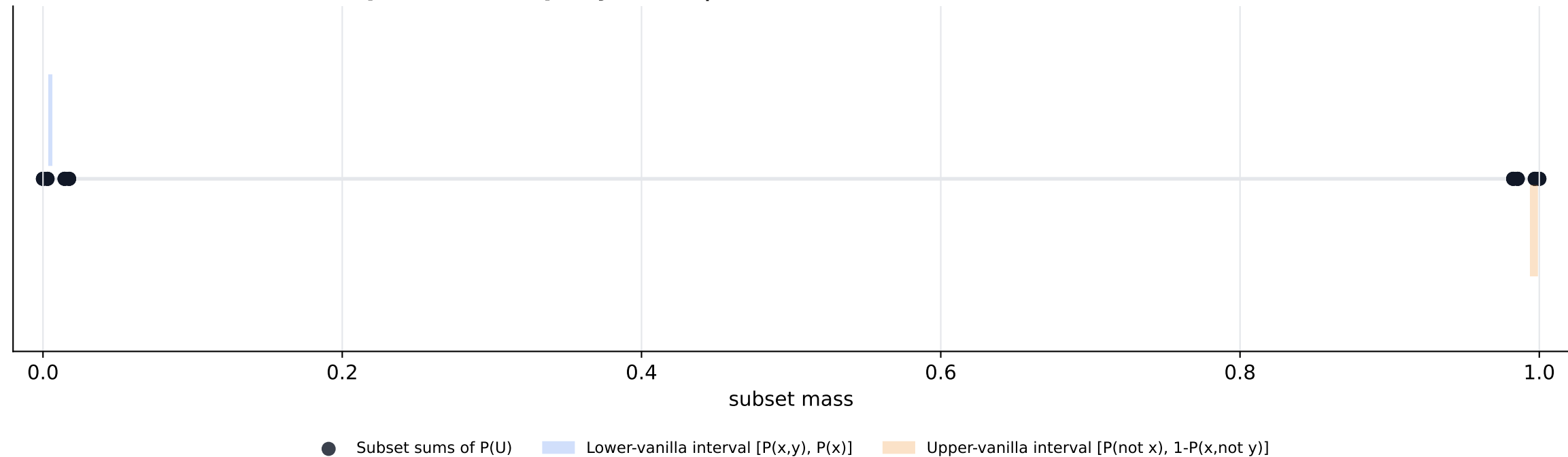
Subset-sum spectrum for query P(Y=0|\text{do}(X=0)) ; H(U)=0.138 bits, distances=(0.00117, 0)
