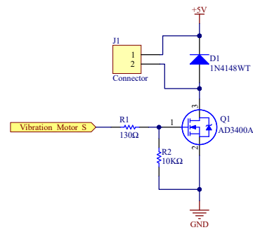
Vibration_Motor
