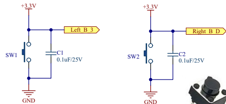
Switch Button
