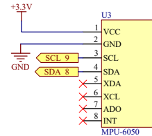
Accelerometer and Gyroscope Sensor
