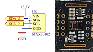
Heart Rate, SpO2, Temperature Sensor
