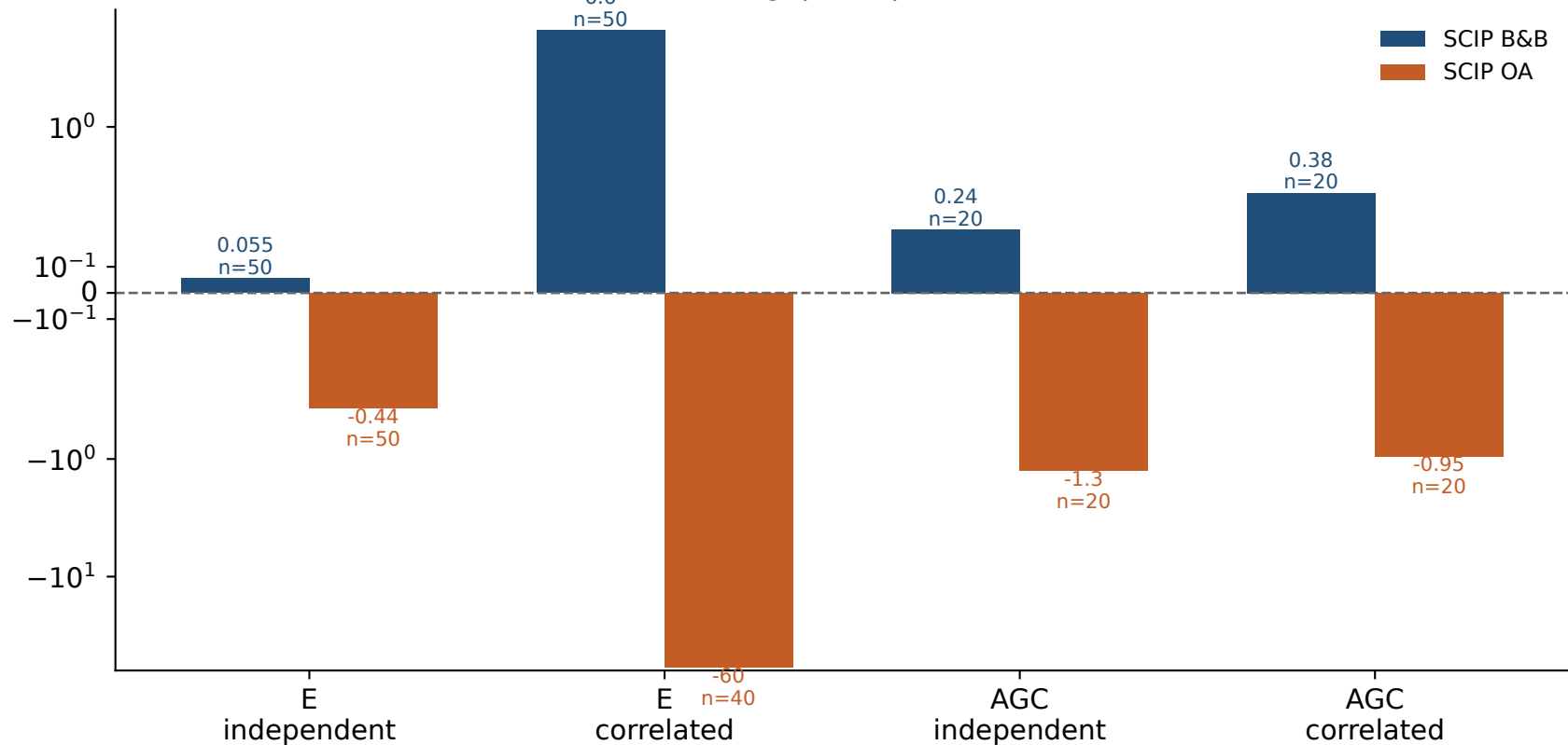
Mean root LB gap vs optimized Boscia
