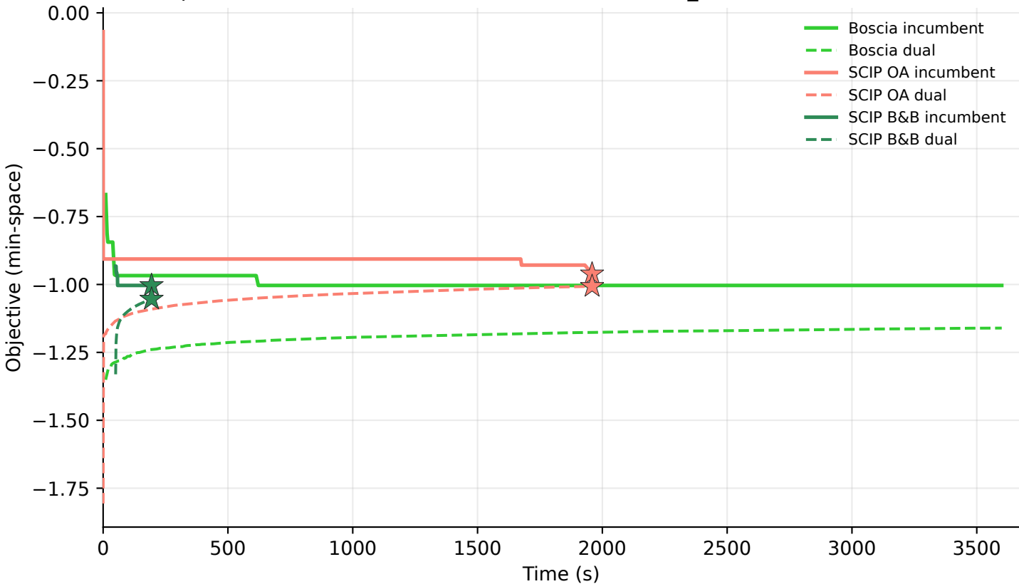
E independent (m=80, N=12, seed=1) — Boscia TIME_LIMIT · SCIP B&amp;B/OA OPTIMAL
