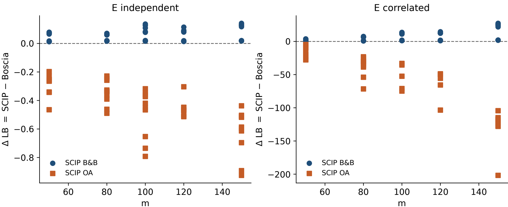
E: root LB gap vs dimension (optimized Boscia)
