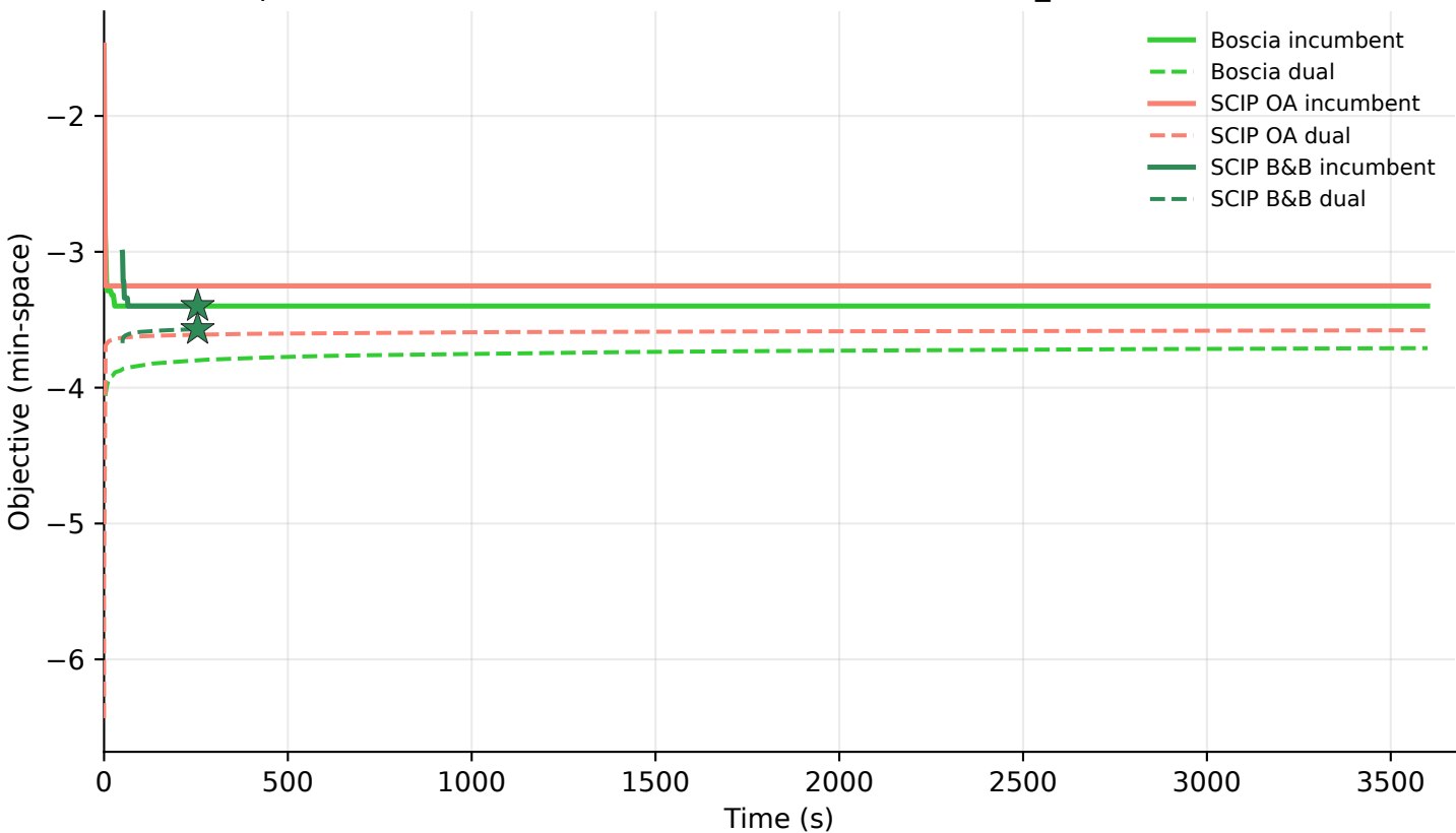
AGC independent (m=80, N=40, seed=3) — Boscia/OA TIME_LIMIT · SCIP B&B OPTIMAL
