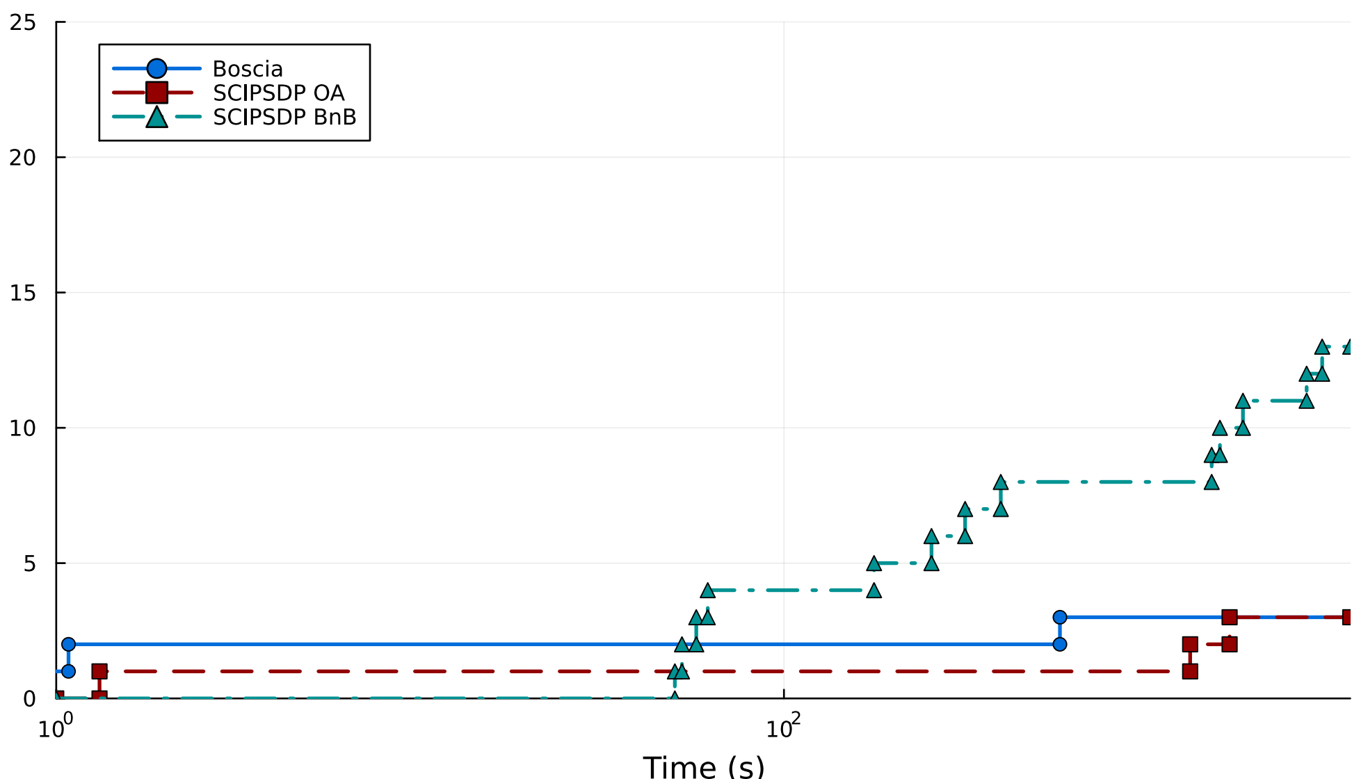
Solved instances
