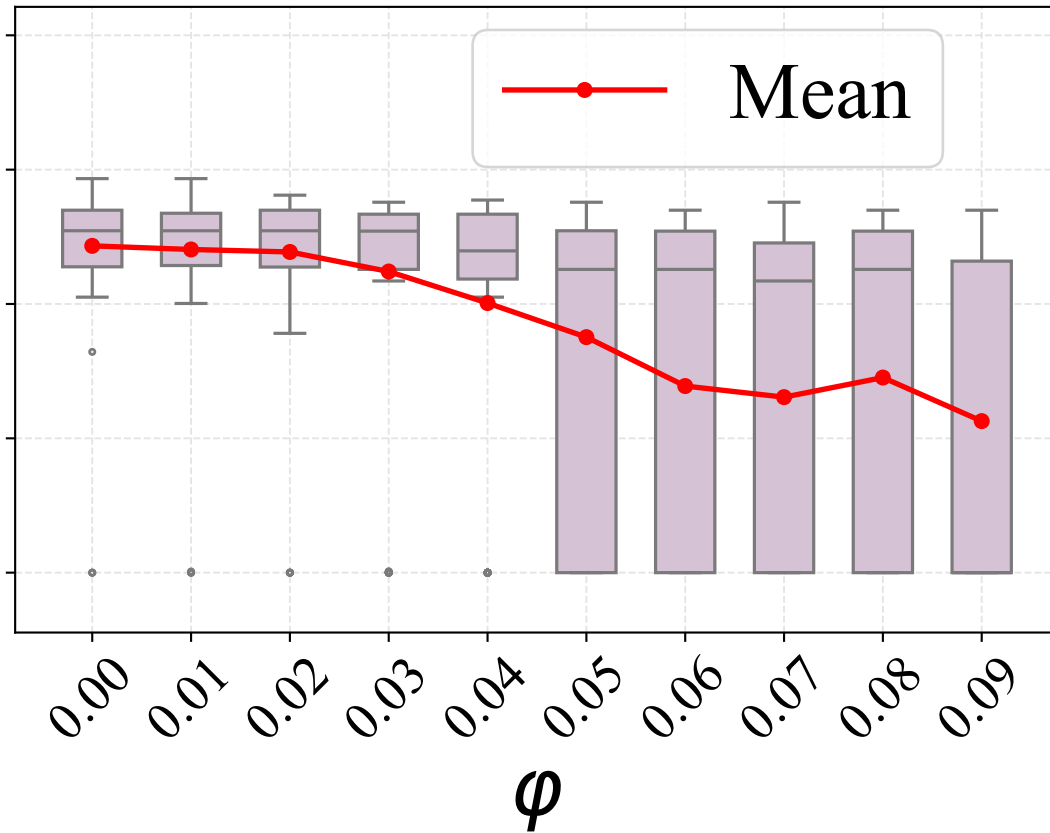
PolBooks
