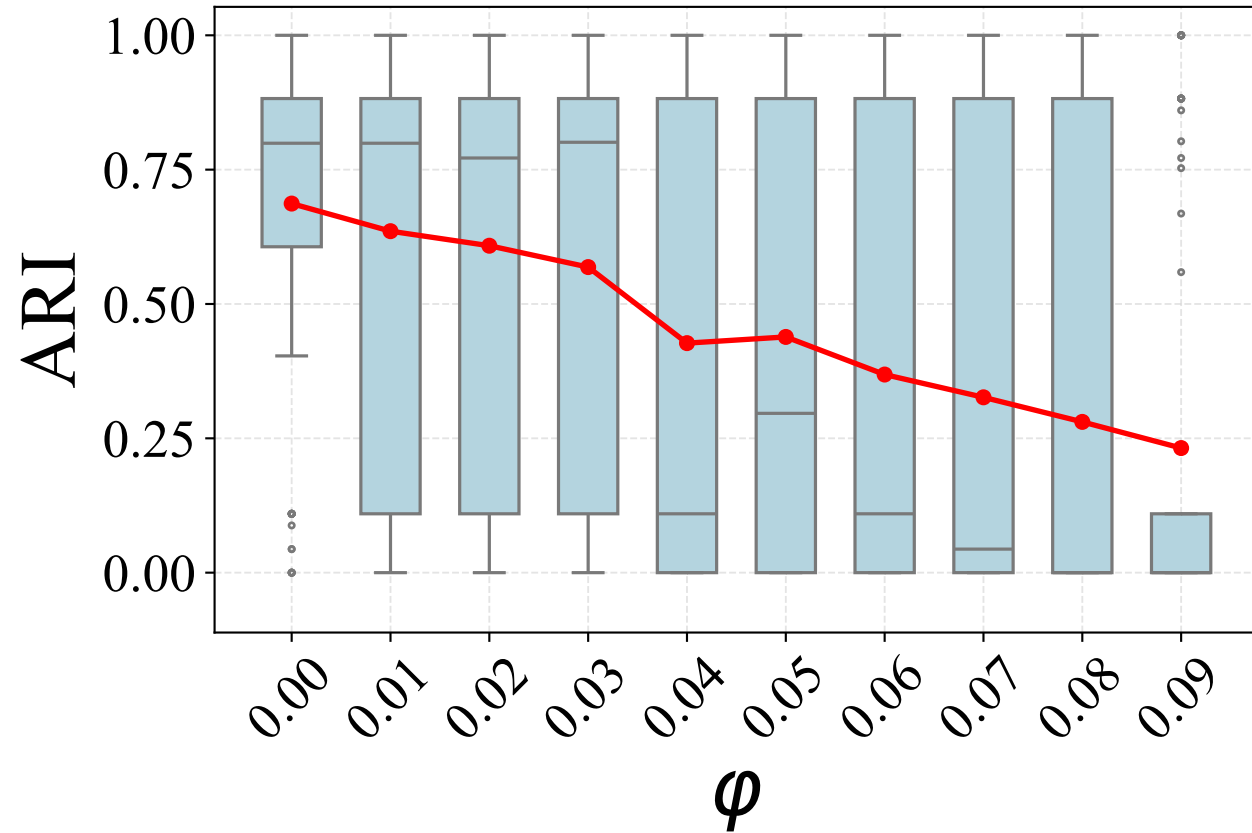
Karate
