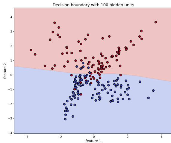
Figure 5: 100 hidden units
