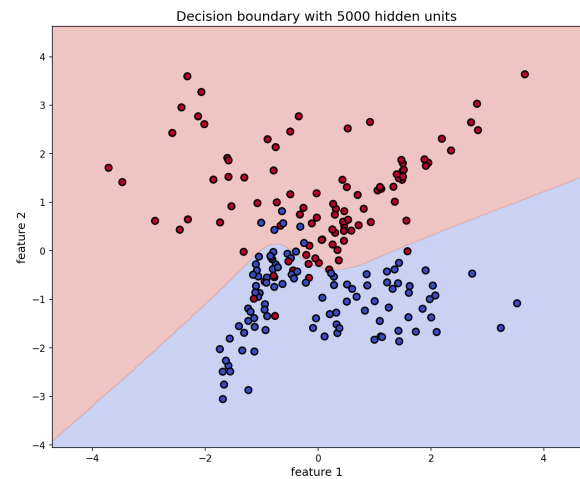
Figure 6: 5000 hidden units
