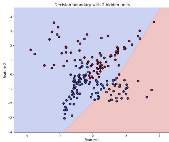
Figure 3: 2 hidden units
