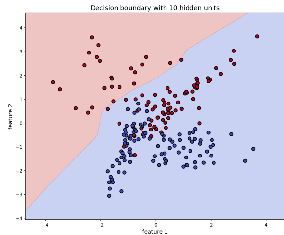
Figure 4: 10 hidden units
