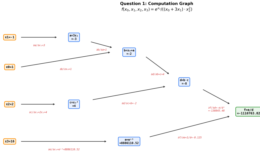
Figure 1: Computation graph of f(x_0, x_1, x_2, x_3) with forward outputs (above edges) and local gradients (below edges).
