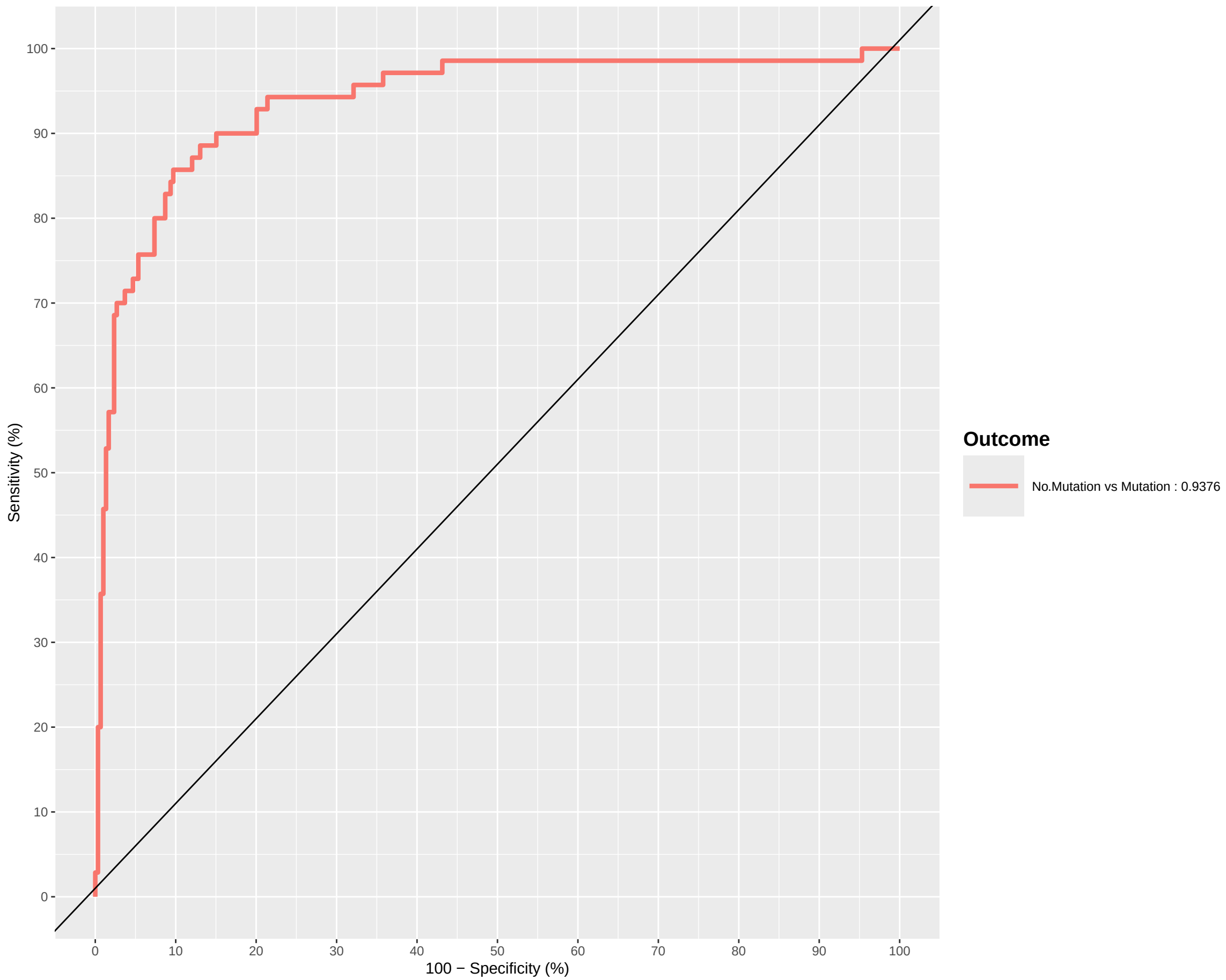
ROC Curve Block: Methyl, Using Comp(s): 1, 2, 3
