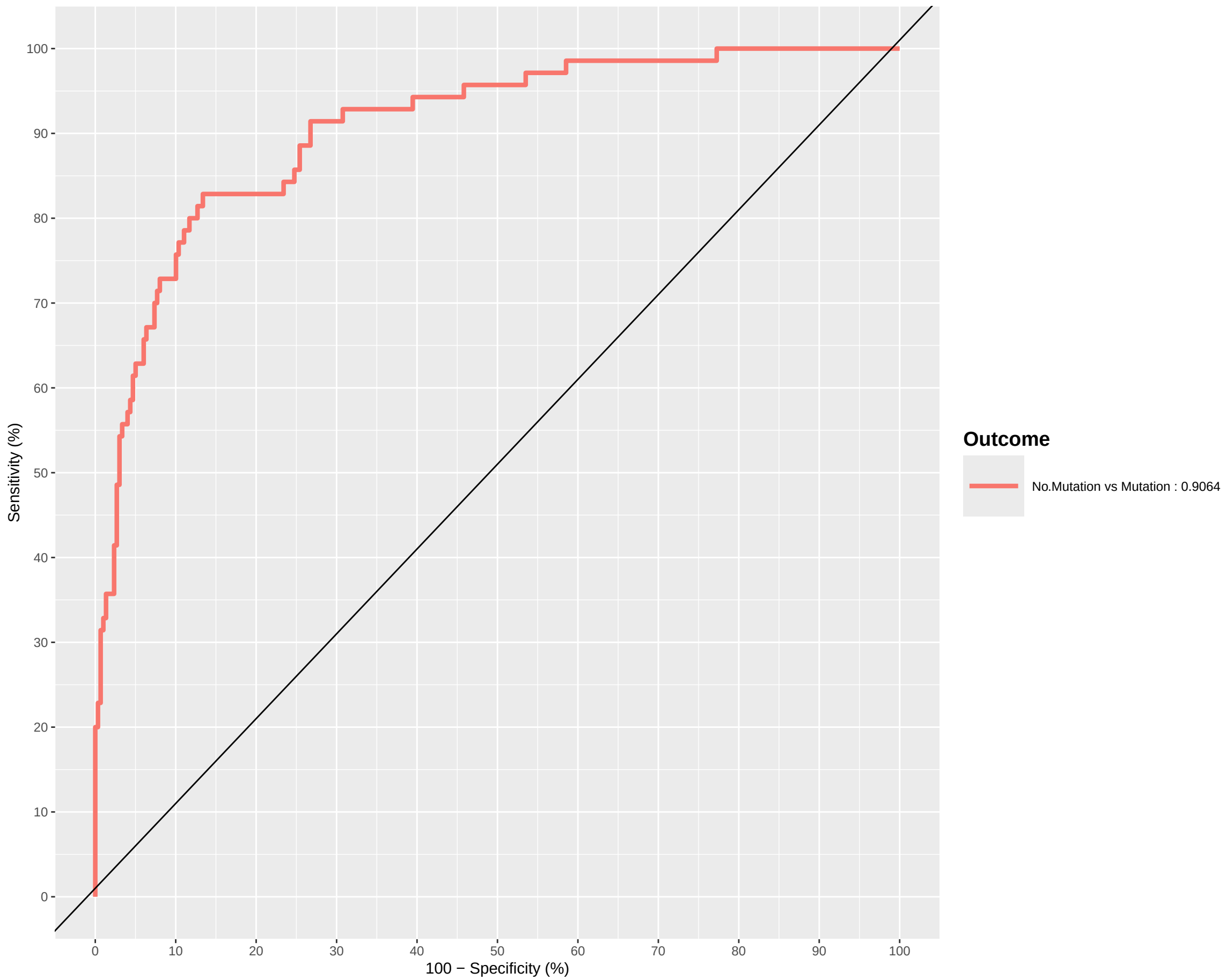
ROC Curve Block: Phospho, Using Comp(s): 1, 2, 3
