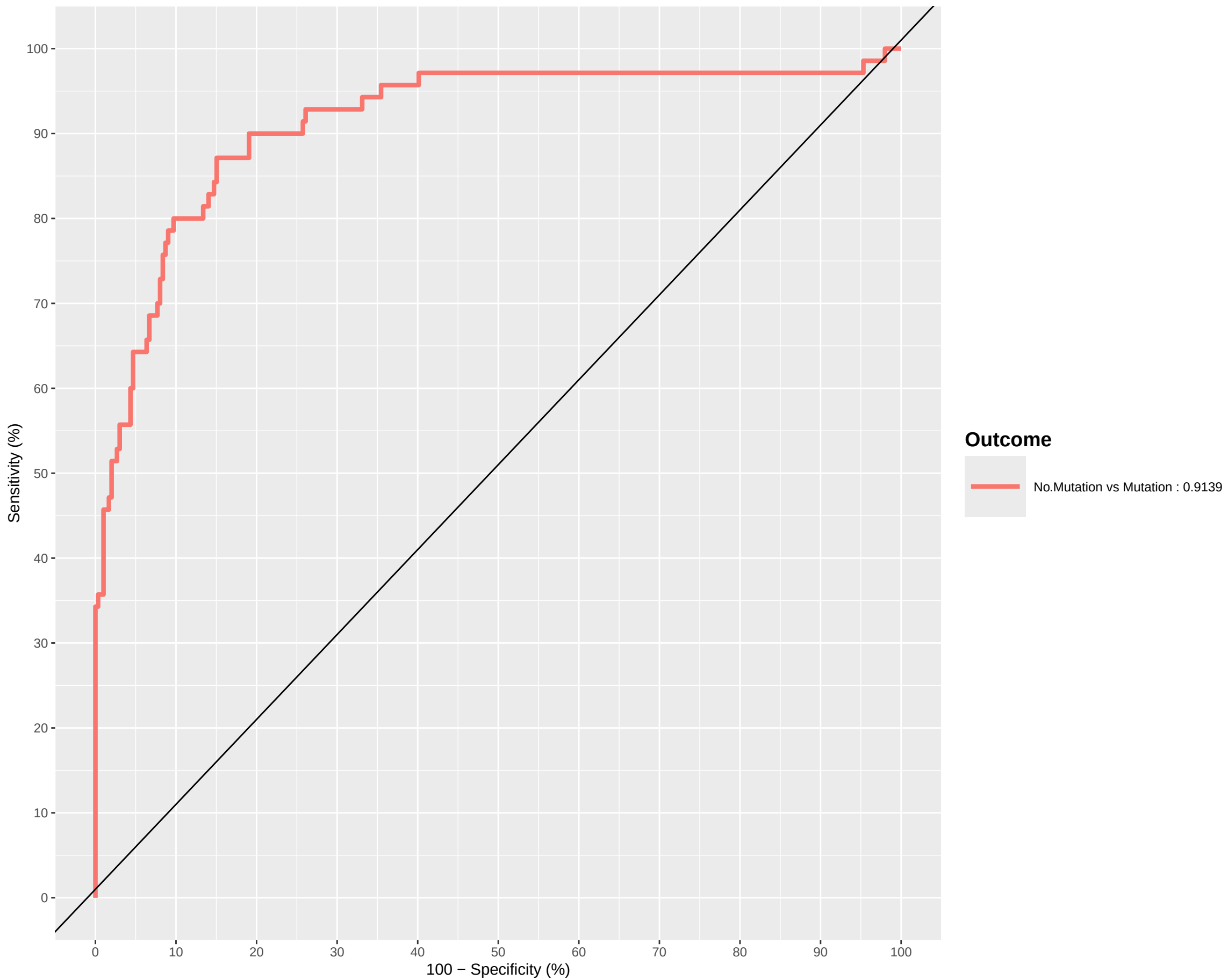
ROC Curve Block: RNA, Using Comp(s): 1, 2, 3
