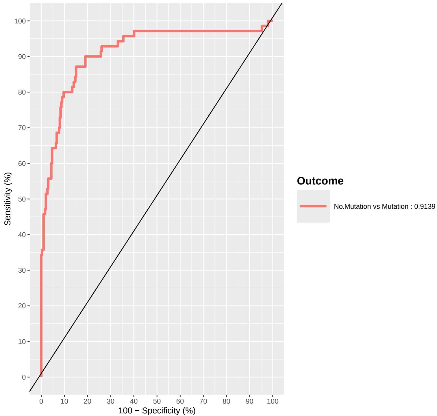
ROC Curve Block: RNA, Using Comp(s): 1, 2, 3
