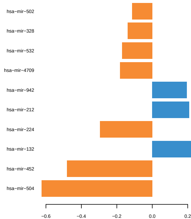
Contribution on comp 2 Block 'miRNA'
