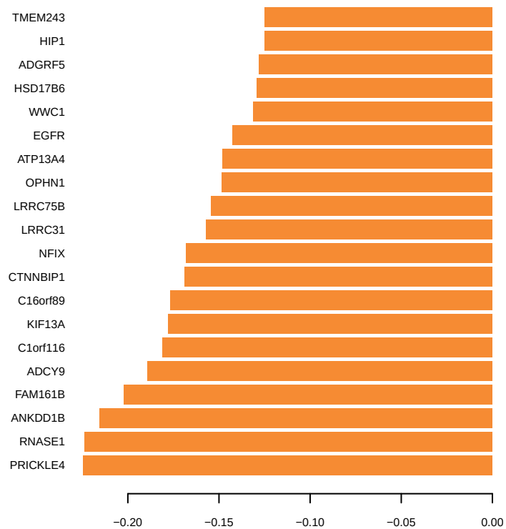
Contribution on comp 2 Block 'RNA'
