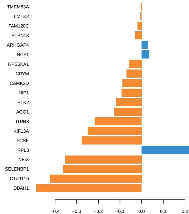
Contribution on comp 2 Block 'Protein'
