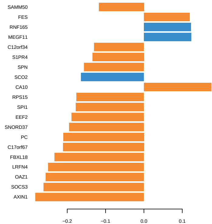
Contribution on comp 2 Block 'Methyl'
