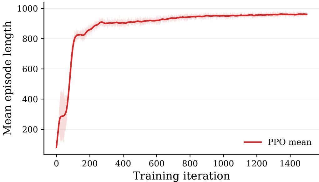
PPO Episode Length Curve
