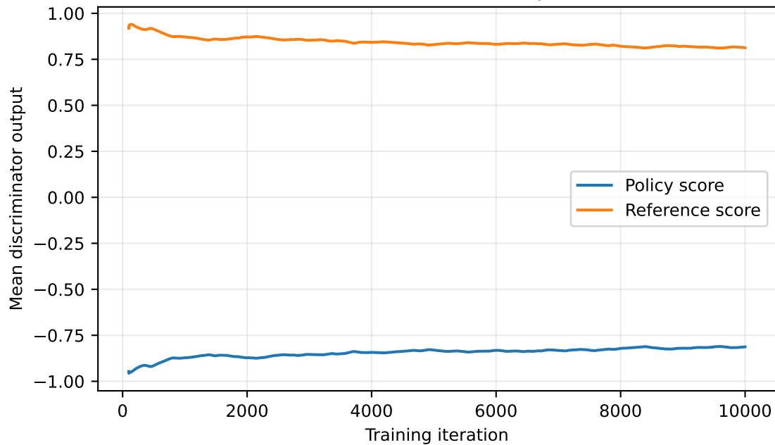
AMP discriminator outputs
