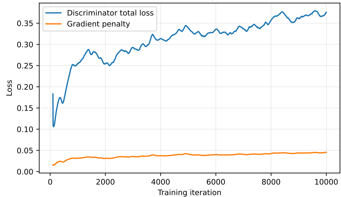
AMP discriminator optimization
