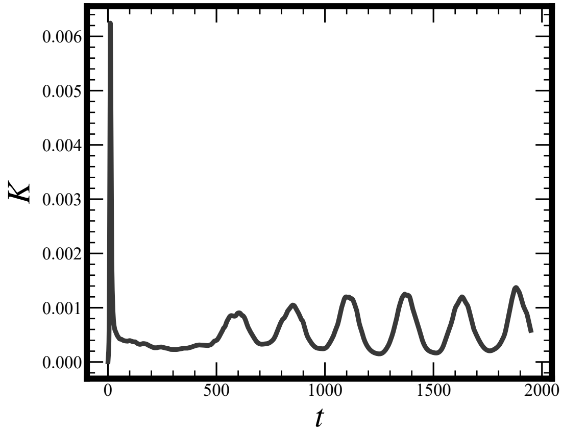
nonrotating, \Gamma = 10
