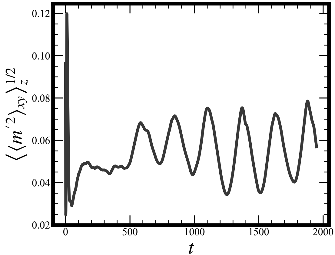
nonrotating, \Gamma = 10
