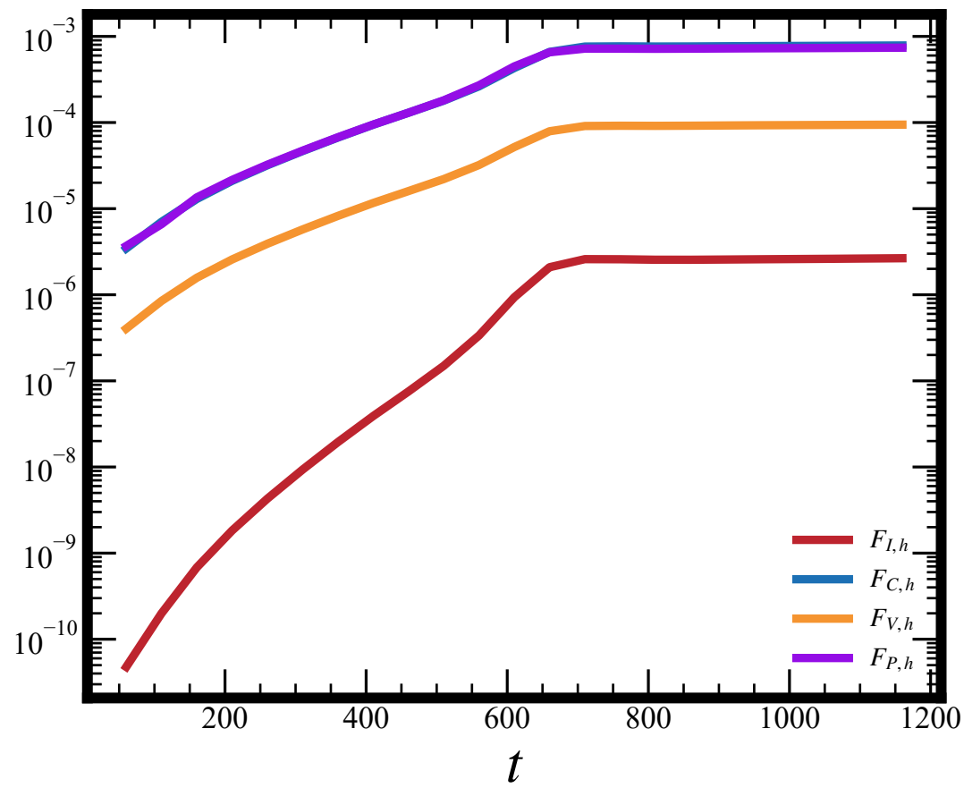
horizontal force at z \simeq 0.048
