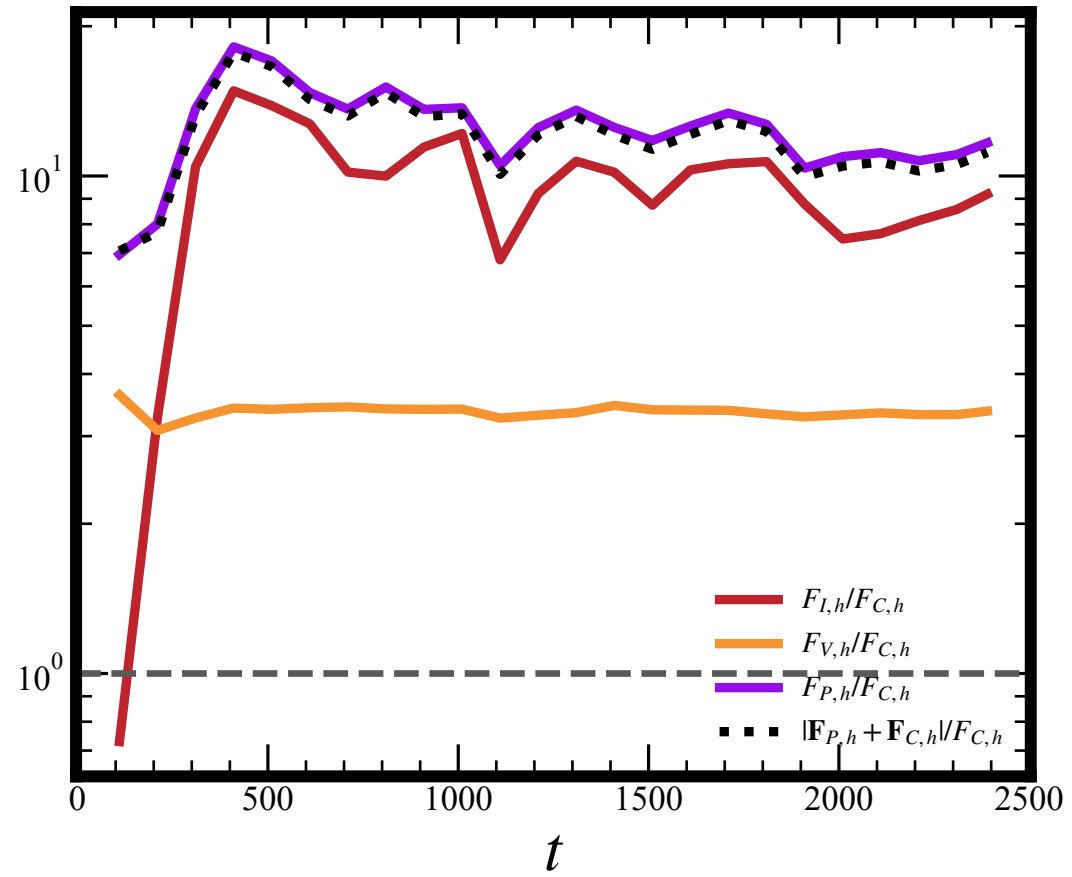
horizontal force ratio
