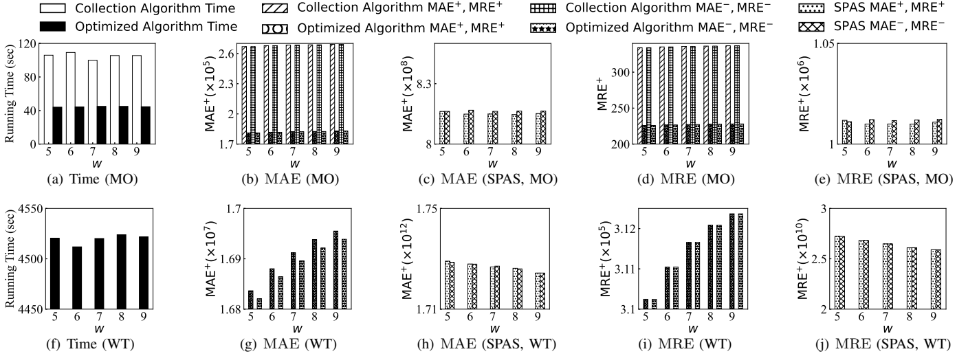
Fig. 12: Impact of window length w
