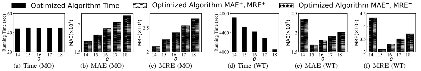
Fig. 13: Impact of step size \theta
