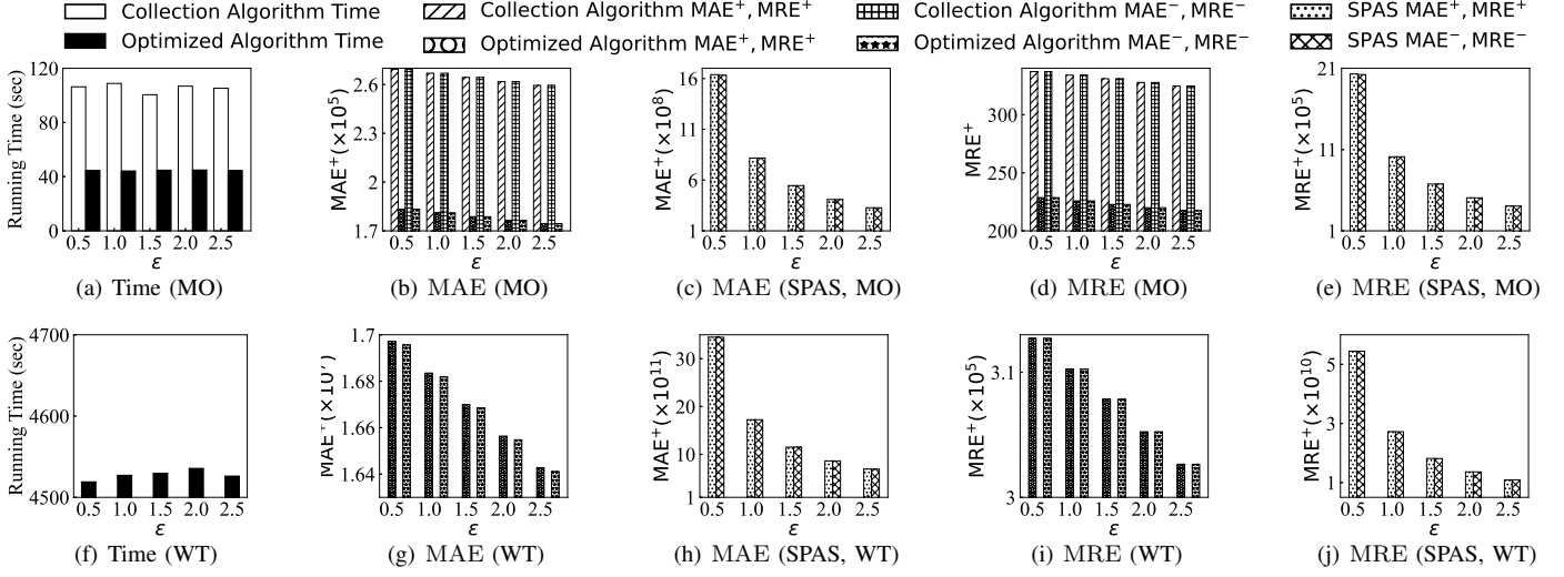
Fig. 11: Impact of privacy budget \epsilon
