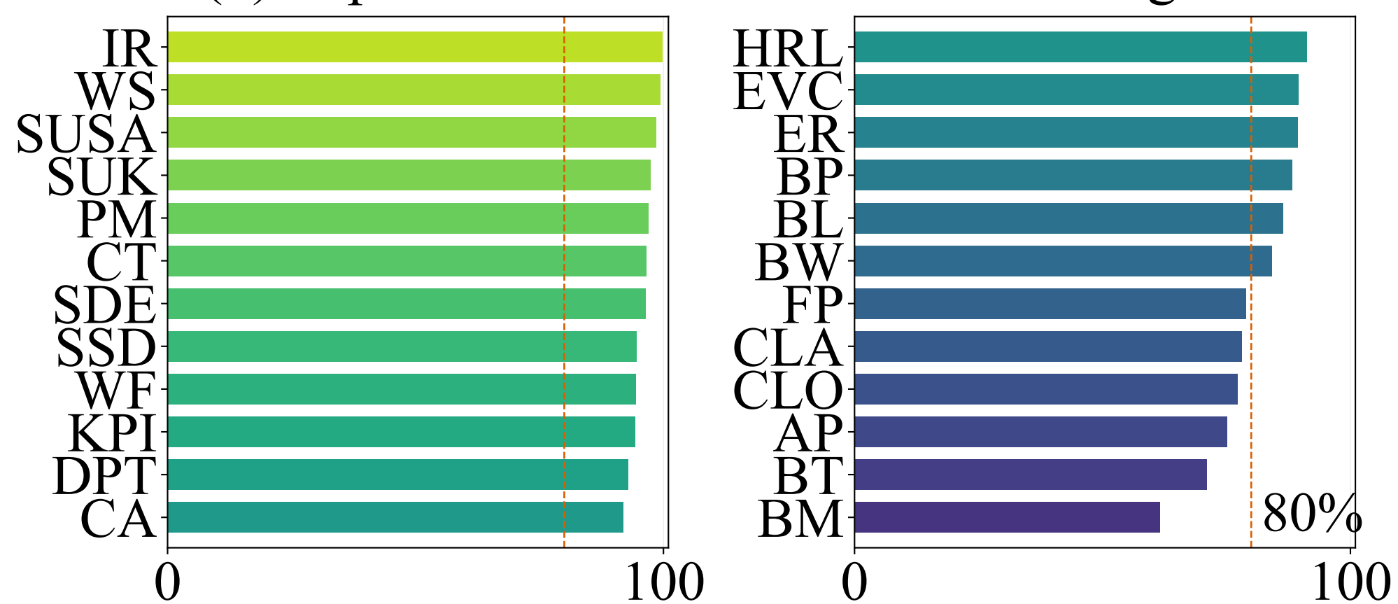
(b) Top 32 Structural Transition Coverage
