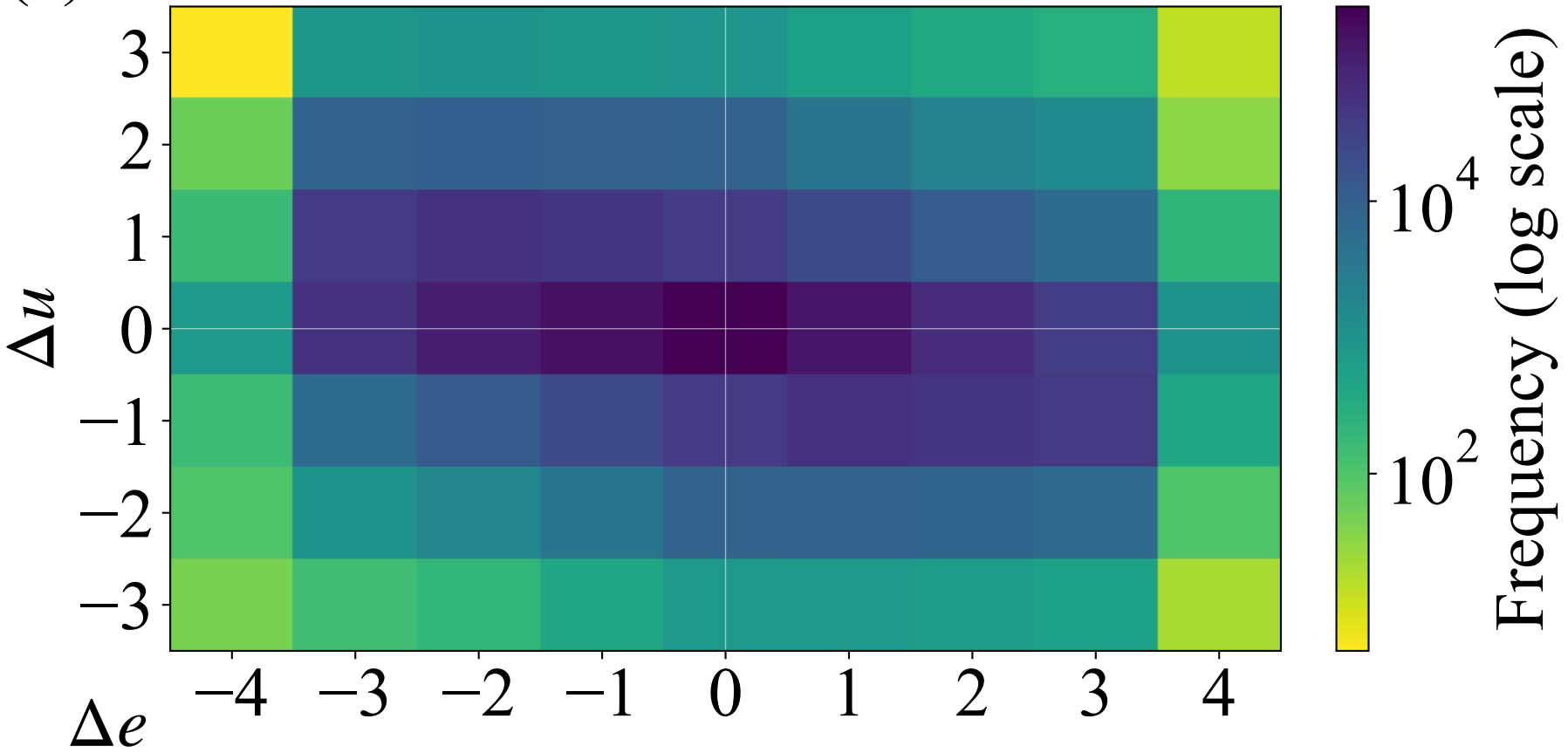
(a) Structural Transition Concentration in SUSa
