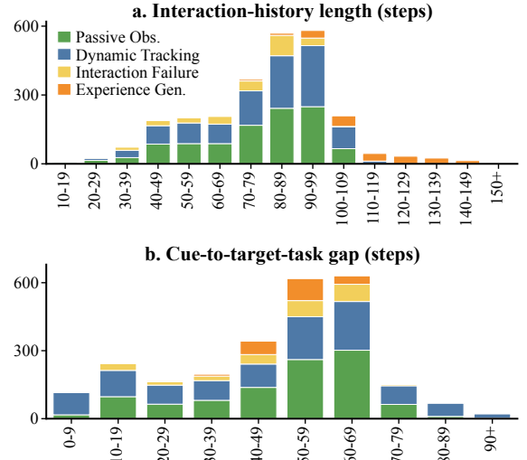
Figure 5 Distributions of interaction-history length and cue-to-target-task distance.
