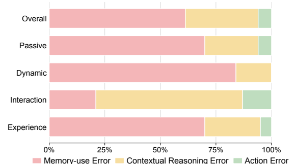
Figure 7 Error distribution of GPT-5.4-mini failures.
