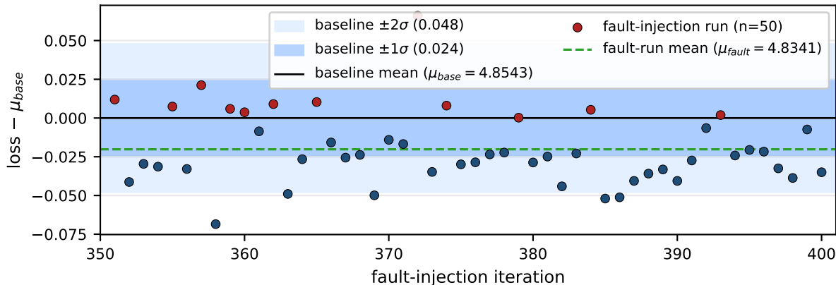
(b) 50 single-fault runs vs 10-run NoFault baseline (44/50 within \pm 2\sigma , 23/50 within \pm 1\sigma )
