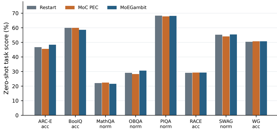
(a) Task scores at step 10,000
