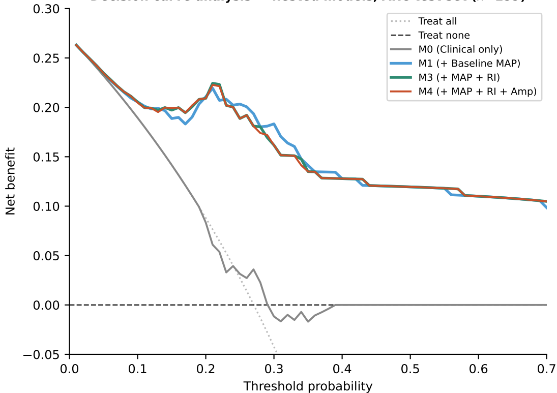
Decision curve analysis — nested models, ARC test set ( n=159 )
