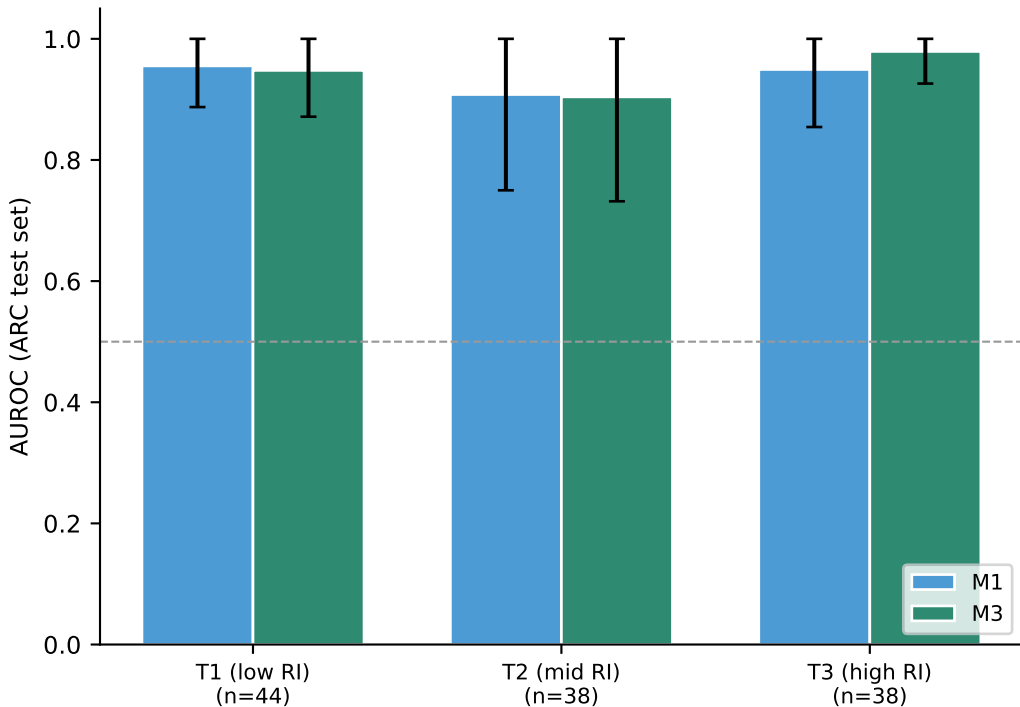
M1 vs M3 AUROC stratified by reflection-index tertile (ARC test) RI adds no discrimination within any tertile
