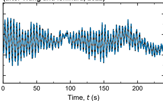
OpenFAST with FounDyn (after Wang and Ishihara, 2022)
