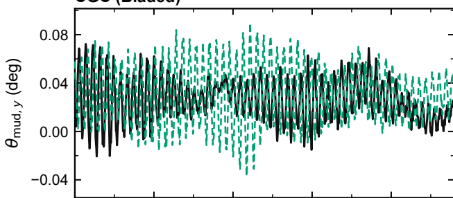
CGC (Bladed)
