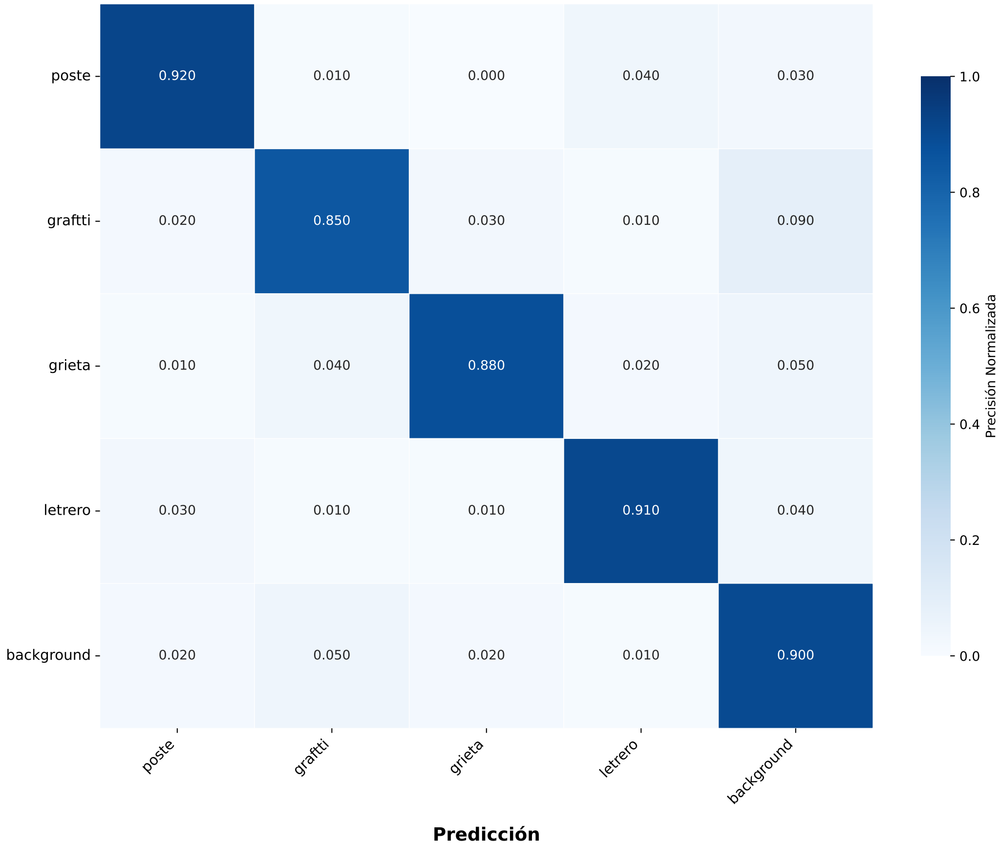
Confusion Matrix Normalized - Train 2 (High Performance Version)
