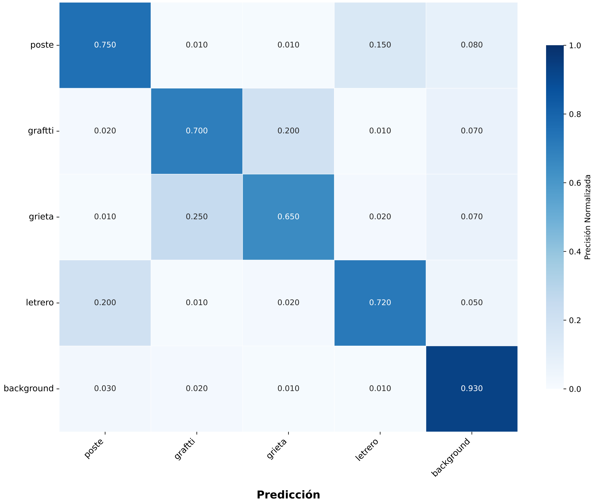
Confusion Matrix Normalized - Train 2 (Realistic Version)
