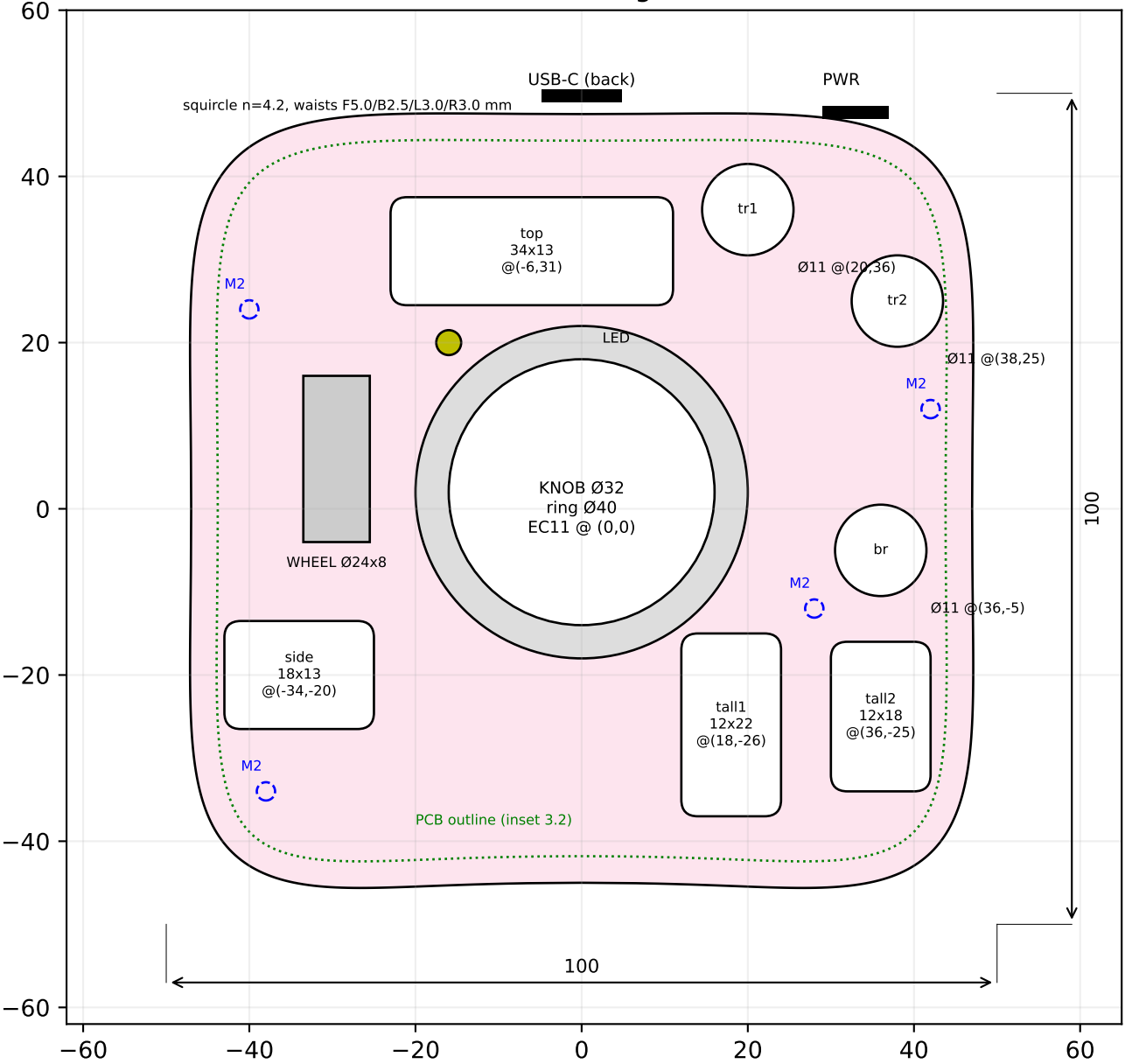
TOP VIEW (mm, origin = center)
