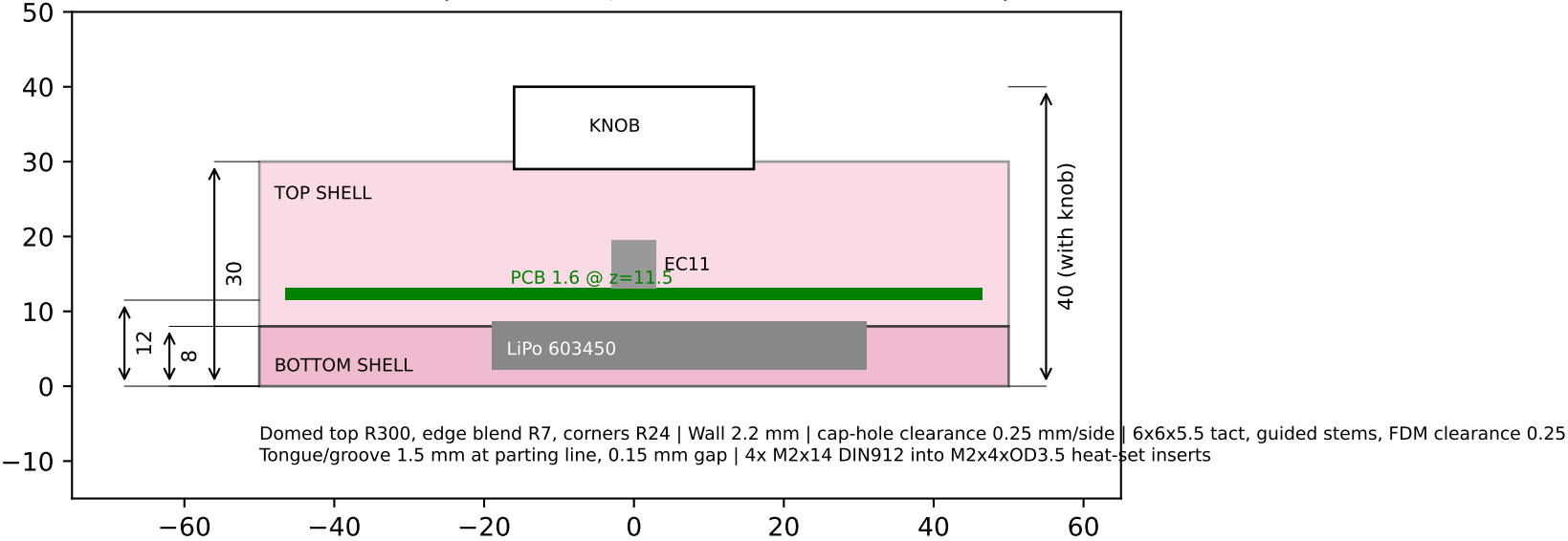
FRONT SECTION (schematic, not to scale for internals)
