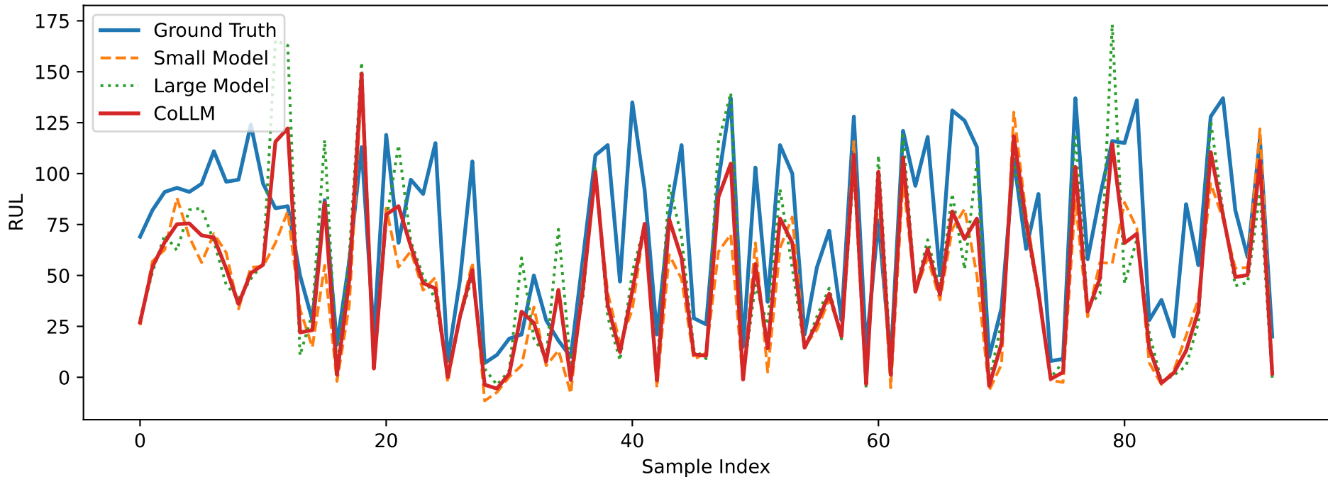
RUL Prediction on Test Set (FD001)
