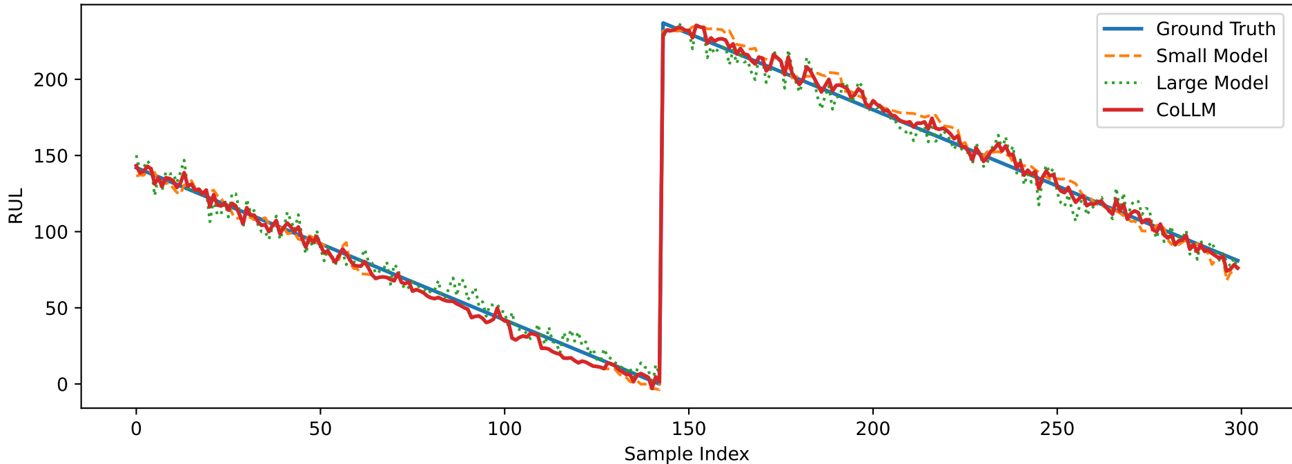
RUL Prediction Comparison (FD001)
