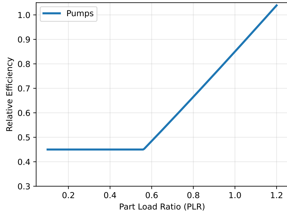
Part-Load Efficiency Curve: Pumps
