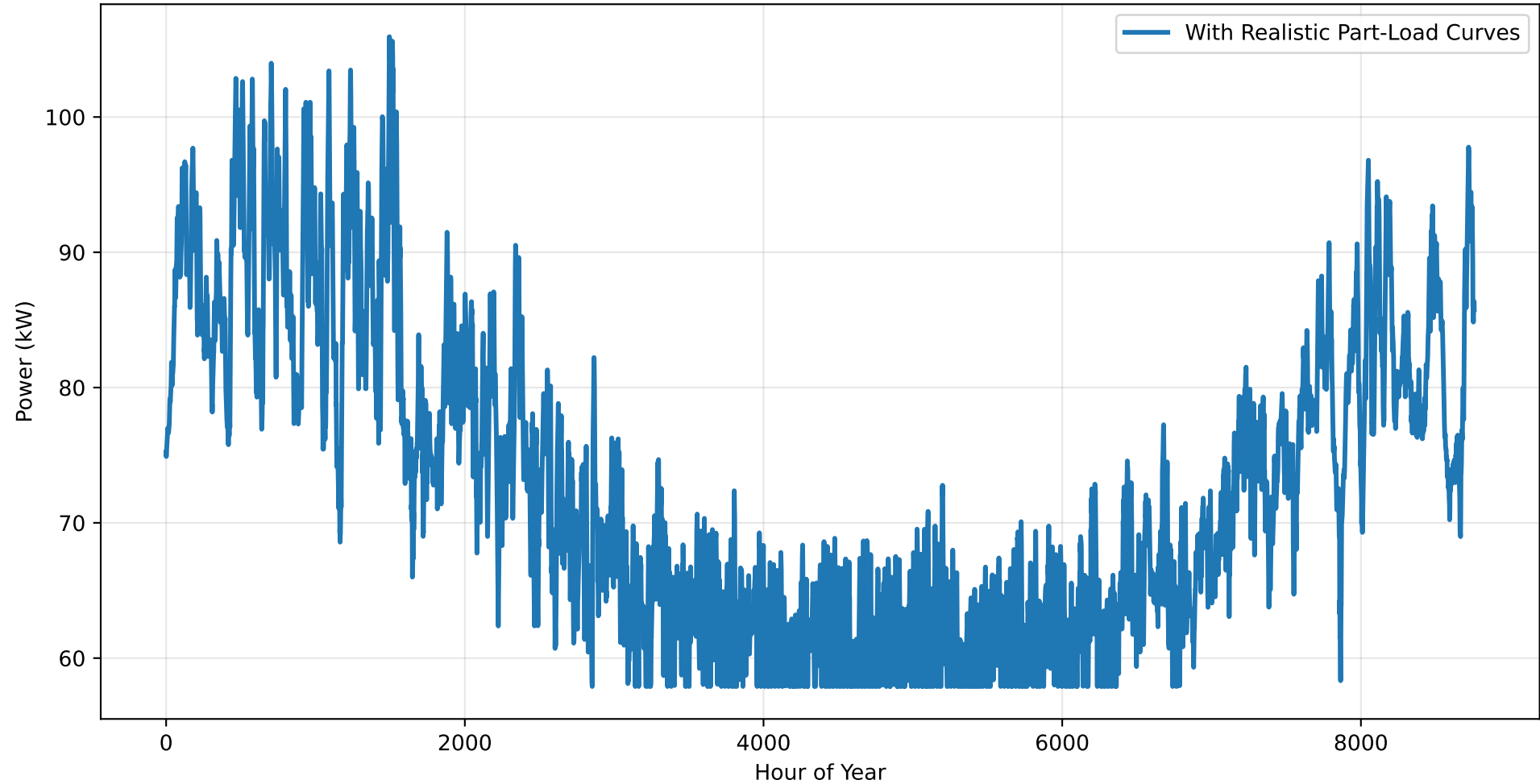
Impact of Part-Load Curves on Baseline Energy
