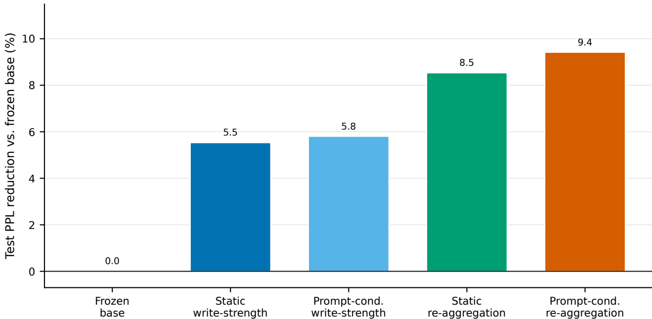
Relative improvement over the frozen base model
