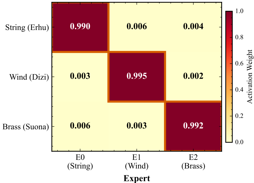
Router Activation Heatmap (50 Epochs, CE Loss)
