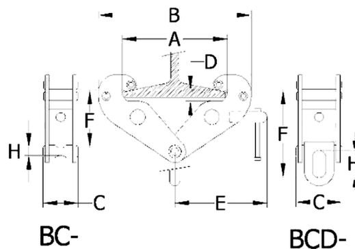
BC (WITHOUT SHACKLE) · BCD (WITH MOVABLE SHACKLE)
