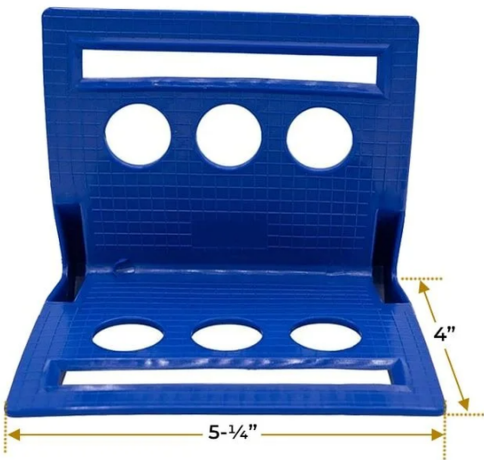
4" PLASTIC CORNER PROTECTOR · 4" × 5-1/4" · FITS 2"–4" WEBBING
