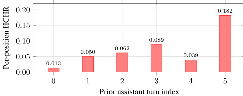
Figure 3: Per-position HCHR on n=80 failed sharded conversations (Qwen2.5-14B). Turn 0 (the first provisional commitment) is almost never solo-flippable. The rate climbs monotonically through turn 3 (0.089), drops at turn 4 ( n=77 ), and spikes at turn 5 ( n=11 , small sample). The mean HCHR across positions is 0.052 with bootstrap CI [0.022, 0.087].
