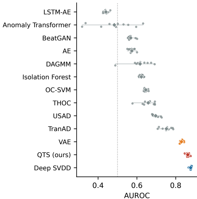
PTB-XL
