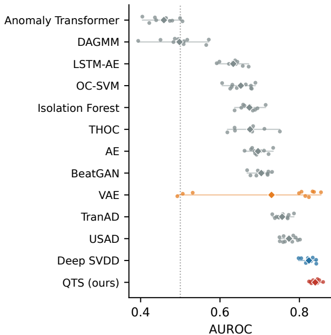
CPSC 2018
