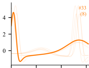
Learned templates ( -w_k , Lead II) | 310 ms = 1 QT interval
