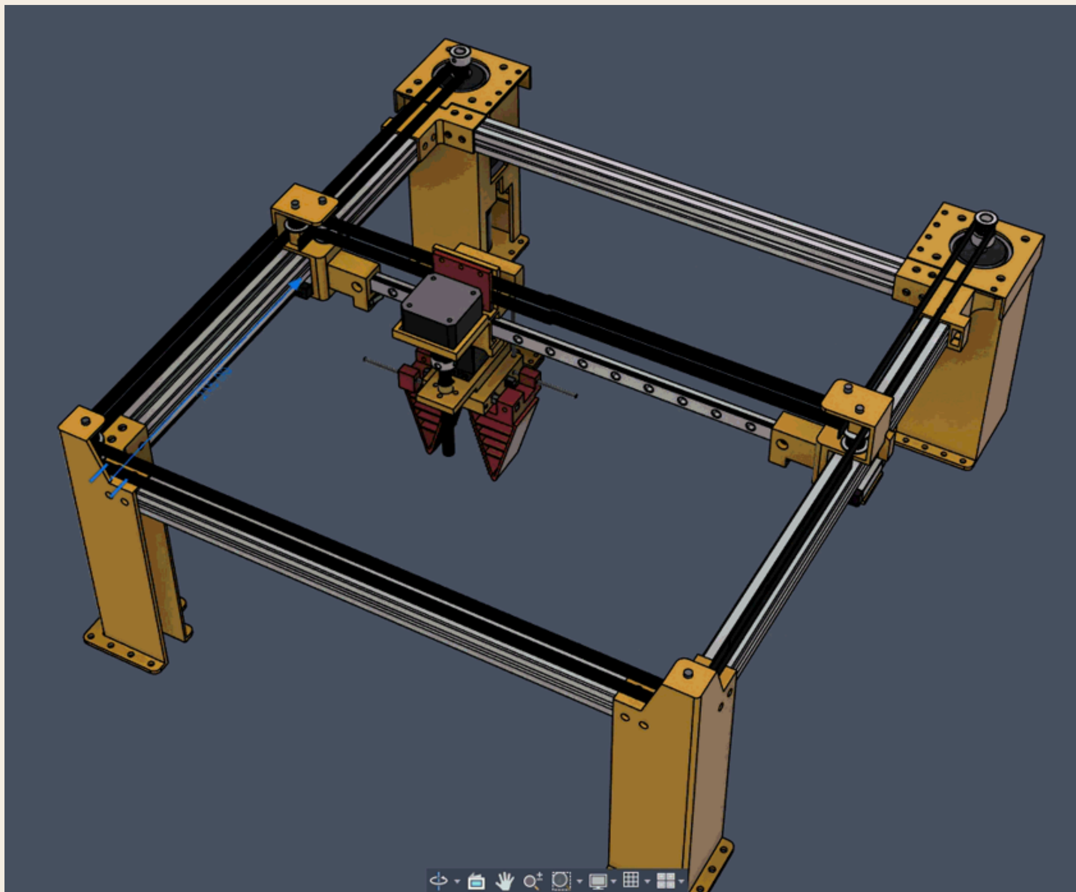
Model robota w 3D - 24.03.2026
