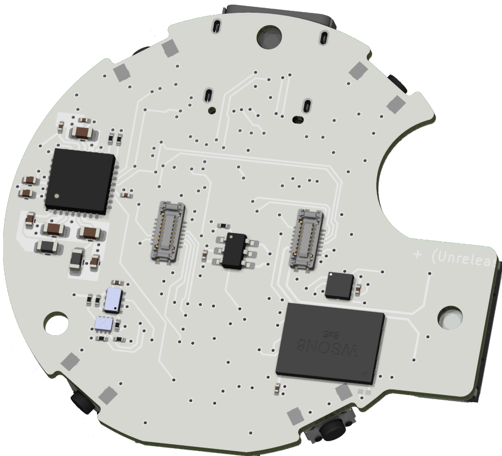
Bottom View
