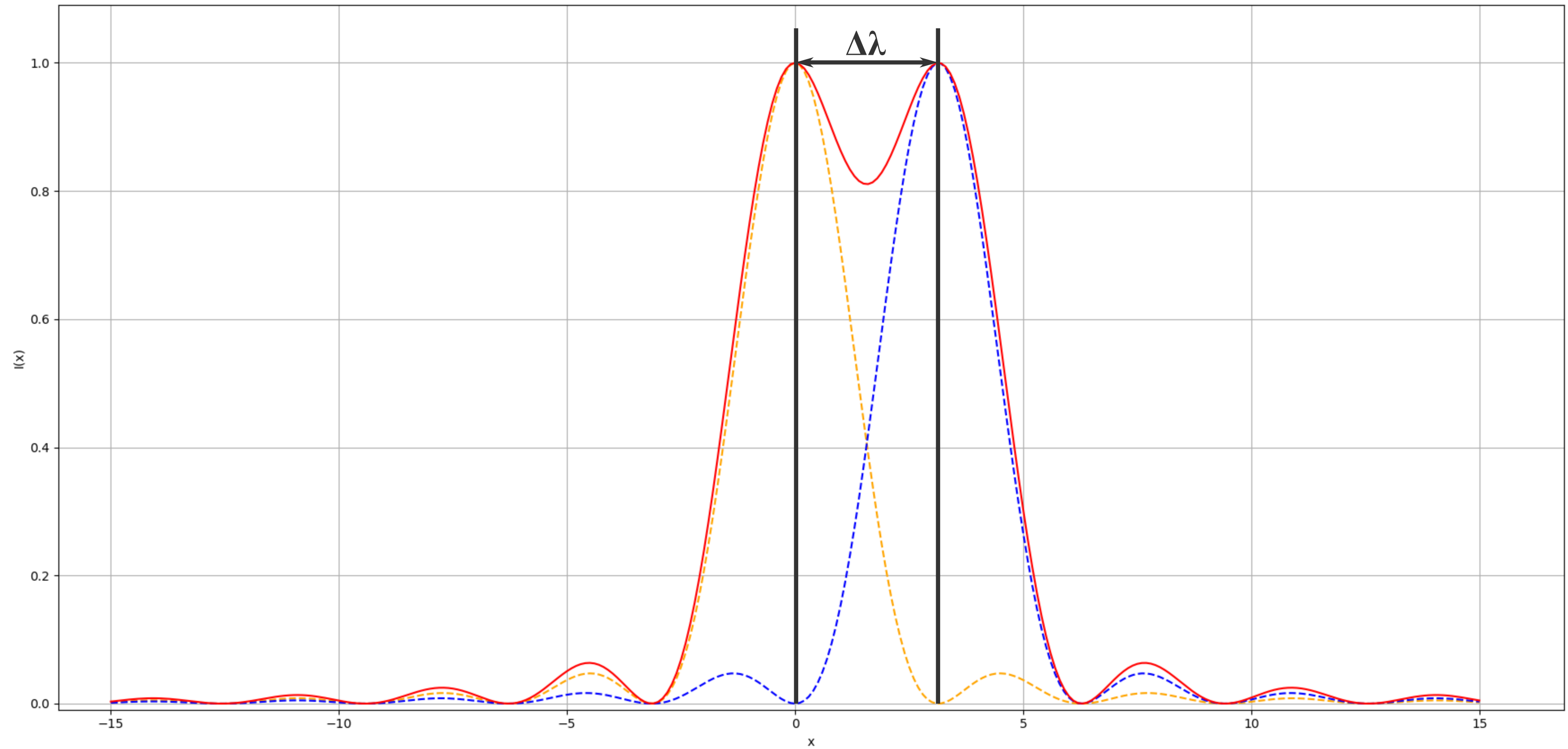
Rayleigh Criterion
