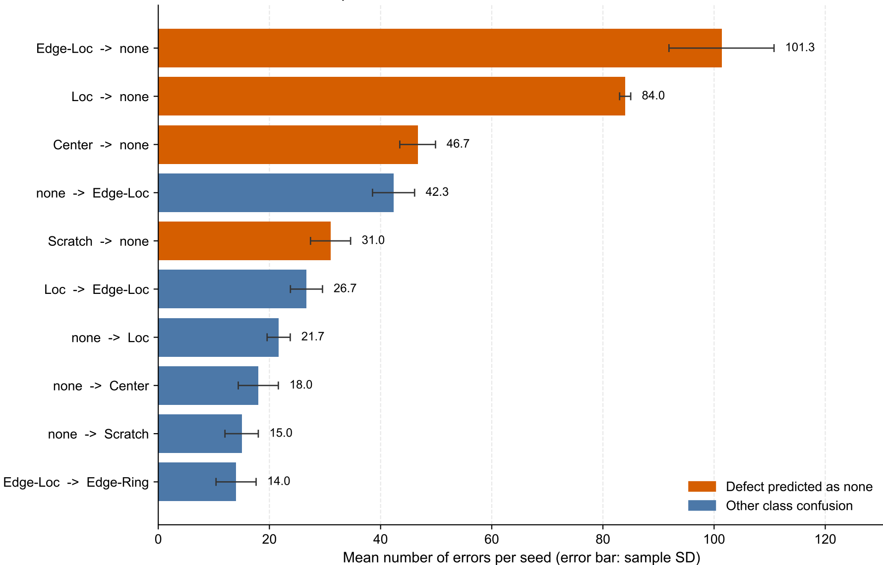
Top Misclassification Directions Across Three Seeds
