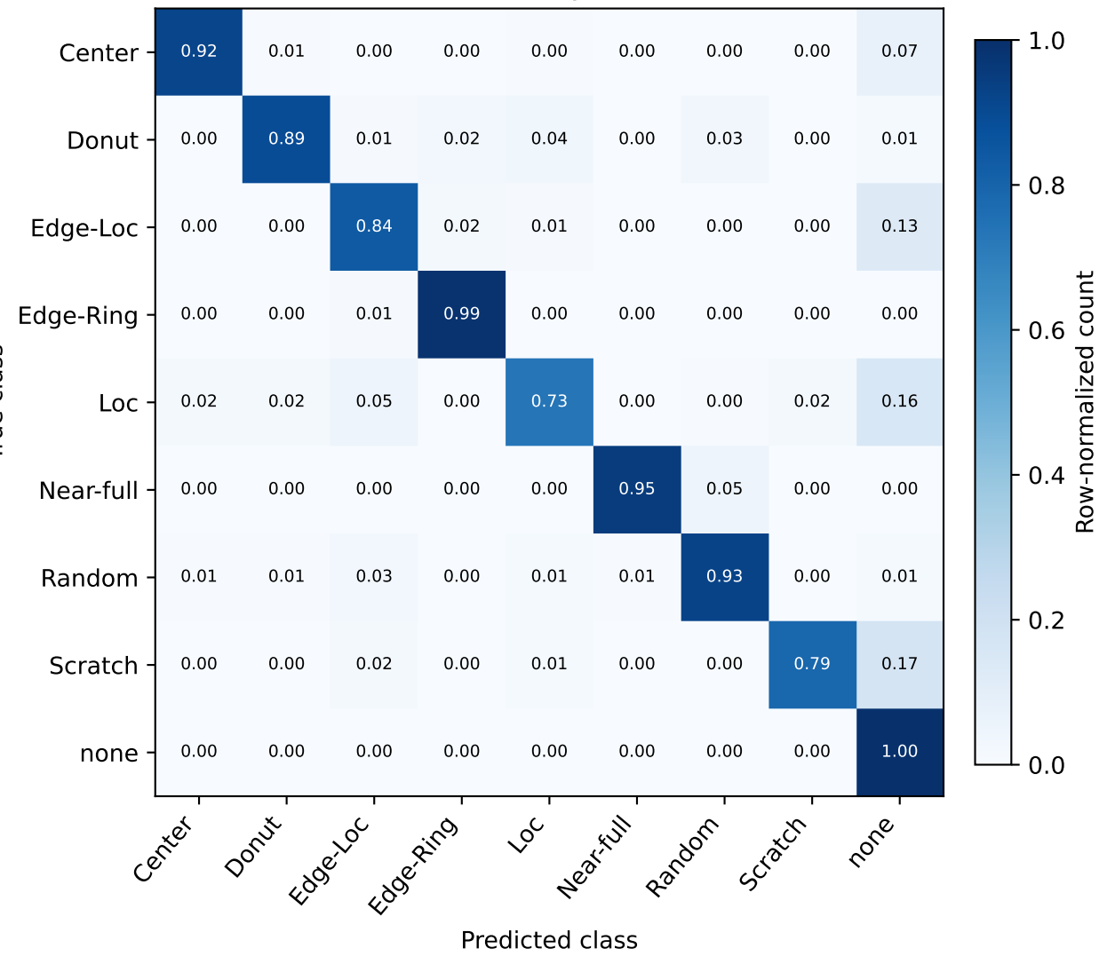
Ordinary CE
