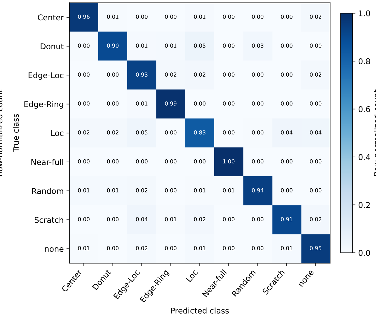
Balanced sampler
