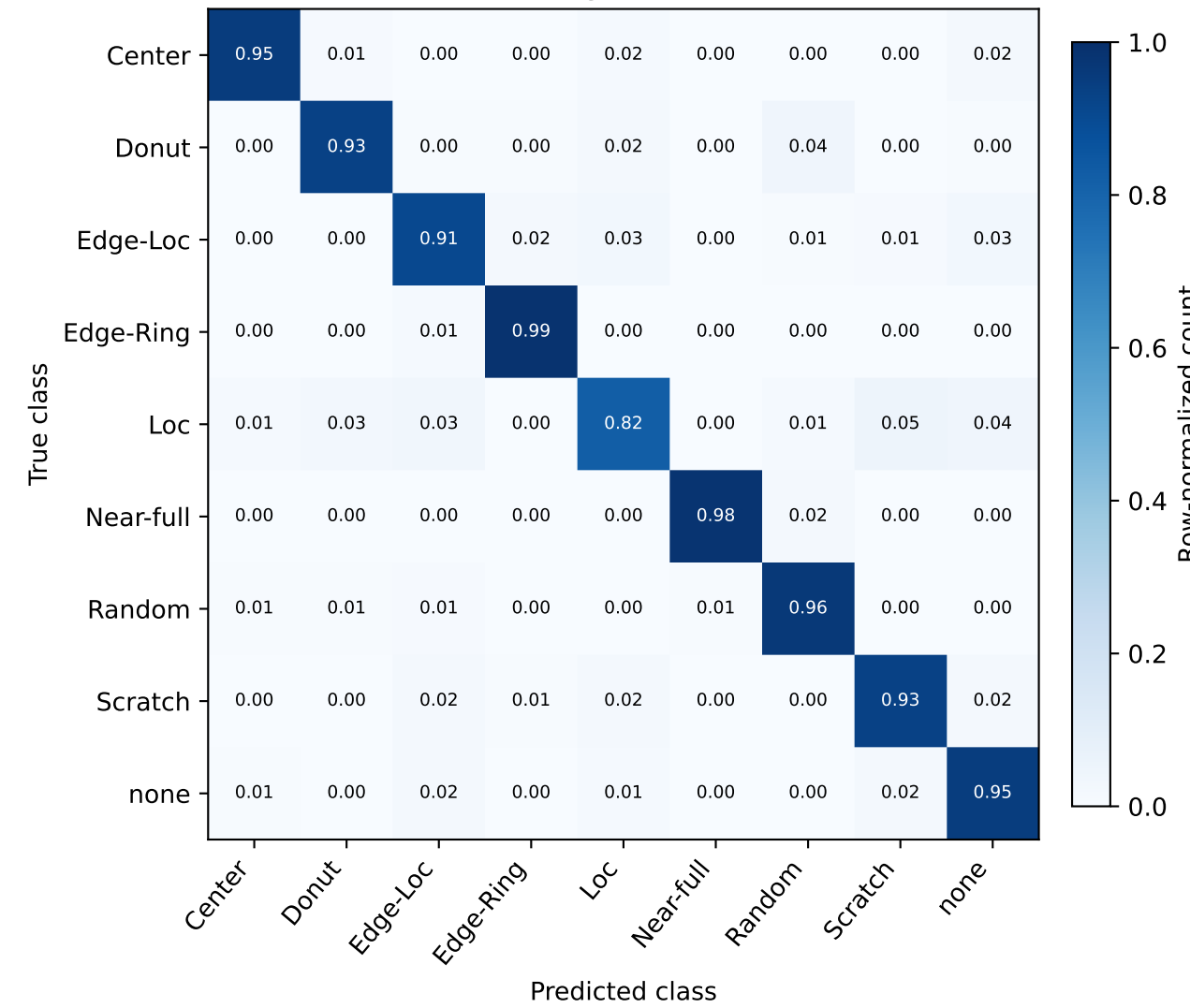
Weighted CE
