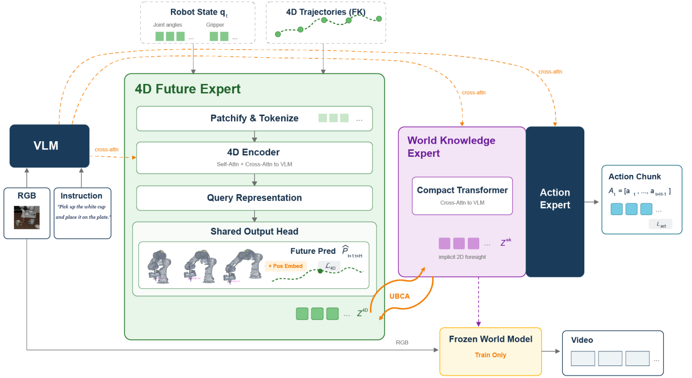
Fig. 1: 4DW-VLA architecture. Robot state q_t and FK-derived 4D trajectories are patchified, tokenized, and fed into the 4D Future Expert , whose 4D Encoder performs self-attention and cross-attention to the VLM prefix. A shared output head predicts both current and future 7D keypoints ( \mathcal{L}_{4D} ). The resulting tokens Z^{4D} are exchanged with the World Knowledge Expert through UBCA, producing implicit 2D-foresight tokens Z^{wk} that supervise a frozen video world model during training only. The Action Expert attends to the VLM, both expert outputs, and generates action chunks ( \mathcal{L}_{act} ). At inference the world model is dropped.
