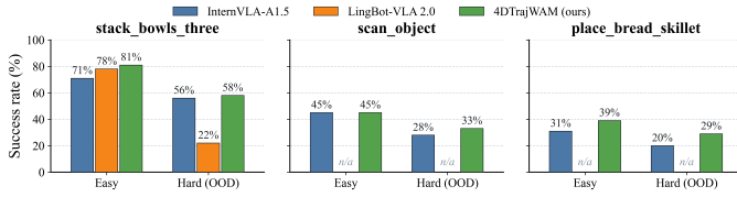
Fig. 2: RoboTwin 2.0 success rates. Grouped bars for Easy and Hard on three tasks. LingBot-VLA 2.0: n/a on two tasks.
