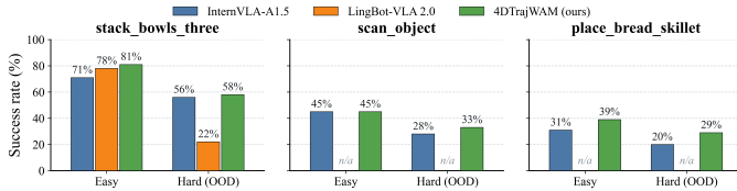
Fig. 3: RoboTwin 2.0 success rates. Grouped bars for Easy and Hard on three tasks. LingBot-VLA 2.0: n/a on two tasks.
